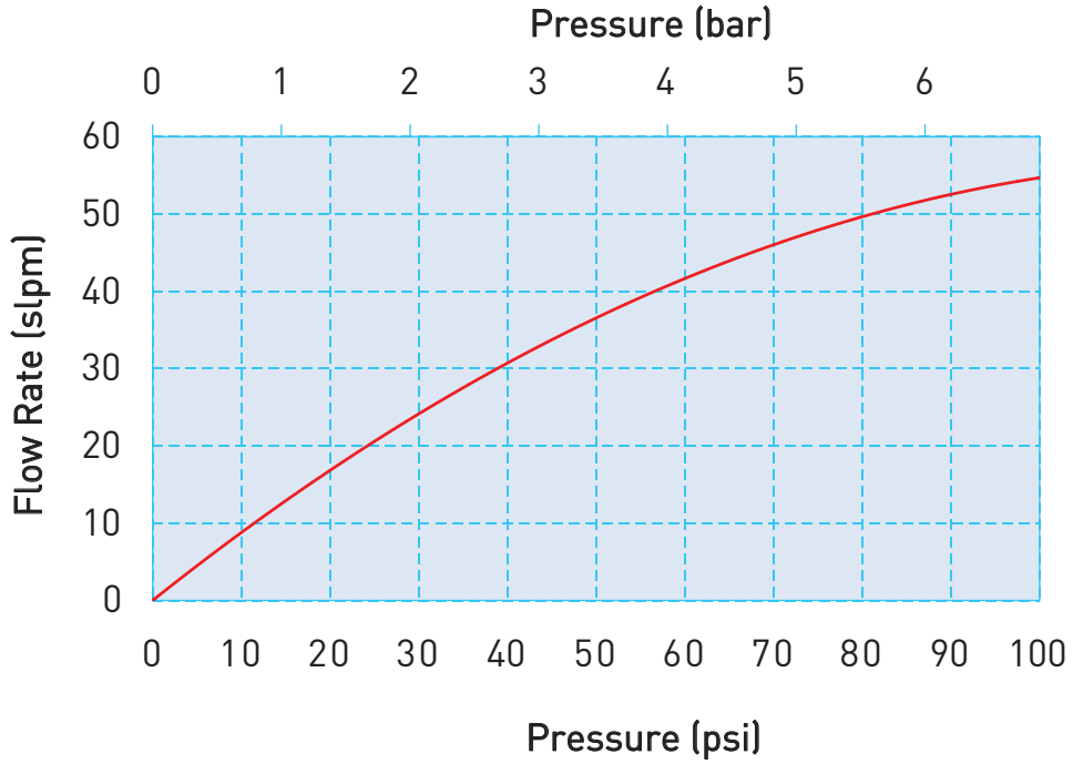
Model 5 - 0.050" (1.27 mm) Orifice
