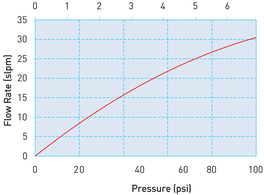
Model 4 - 0.040" (1.02 mm) Orifice Pressure (bar)
